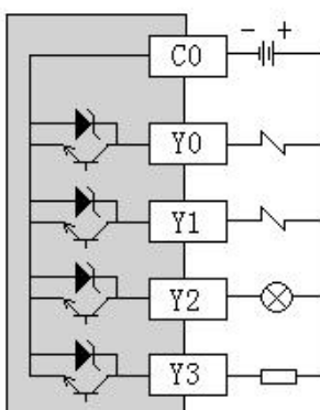
DC NPN Transistor output
